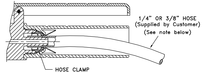
Cross Section View of Handle/Hose Clamp Assembly
